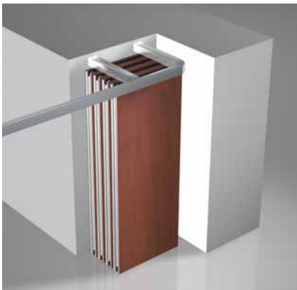
Stacking solution PL3
